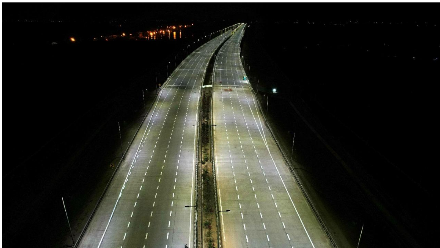
Lighting and road marking completed near Ankleshwar, Gujarat
