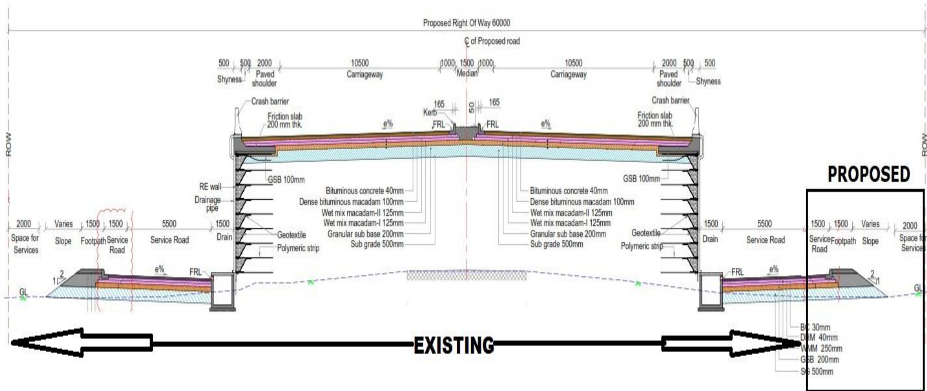
TYPICAL CROSS SECTION -V
