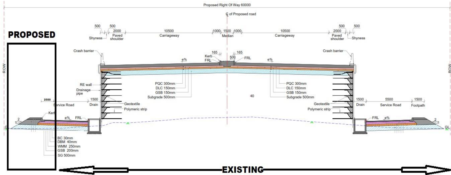
TYPICAL CROSS SECTION - VI
