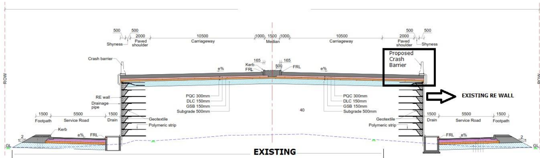
TYPICAL CROSS SECTION - XIV
