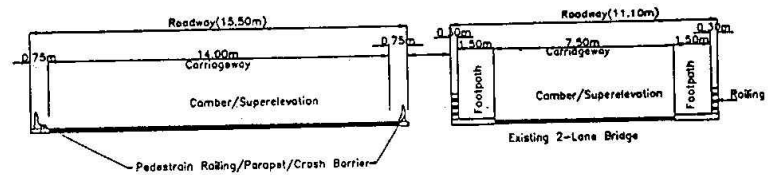
Cross Section of Bridge at Deck Level - With Footpath (T-Beam/Box Girder type/Well/Pile foundation) 4-LANE DIVIDED HIGHWAY ( One side new bridge and other side Existing 2-lane bridge)
