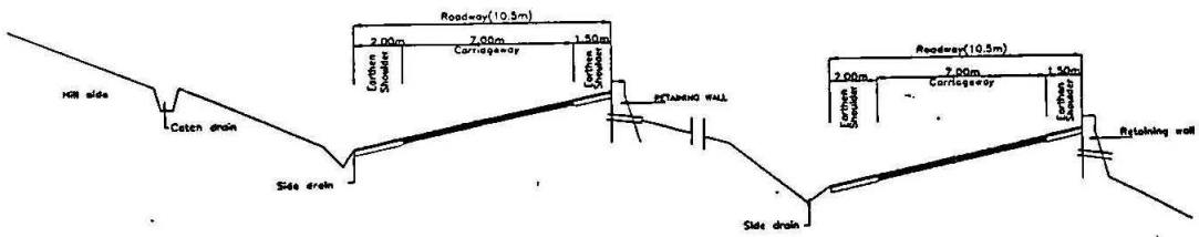
TYPICAL CROSS SECTION TYPE-C1 (Open country - Mountainous terrain) 4-LANE DIVIDED HIGHWAY ON DIFFERENT CONTOURS
