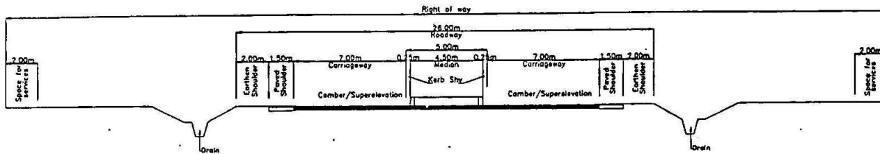
TYPICAL CROSS SECTION TYPE-A3 (Open country—Plain/Rolling terrain) 4-LANE DIVIDED HIGHWAY WITHOUT SERVICE ROADS AND WITH RAISED MEDIAN
