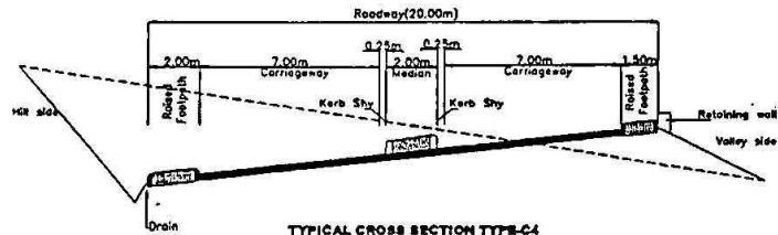
TYPICAL CROSS SECTION TYPE-C4 (Built up section - Mountainous terrain) 4-LANE DIVIDED HIGHWAY AT SAME LEVEL WITH RAISED MEDIAN
