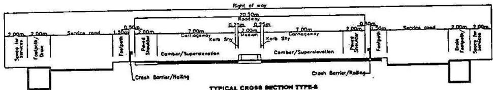
TYPICAL CROSS SECTION TYPE-B (Built-up Section - Plain/Rolling terrain) 4-LANE DIVIDED HIGHWAY WITH SERVICE ROADS AND WITH RAISED MEDIAN
