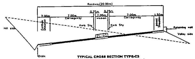
TYPICAL CROSS SECTION TYPE-C3 (Open country - Mountainous terrain) 4-LANE DIVIDED HIGHWAY AT SAME LEVEL WITH RAISED MEDIUM
