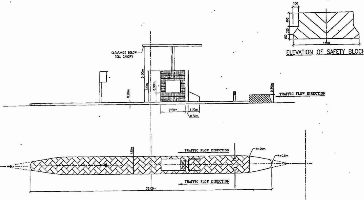
TYPICAL LAYOUT FOR TRAFFIC ISLAND WITH TOLL BOOTH
