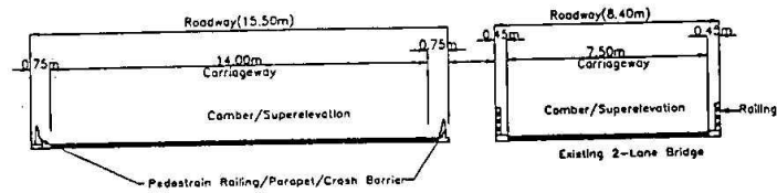
Cross Section of Bridge at Deck Level - Without Footpath (T-Beam/Box Girder type/Well/Pile foundation) 4-LANE DIVIDED HIGHWAY ( One side new bridge and other side Existing 2-lane bridge)
