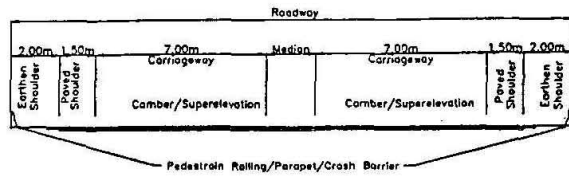
Cross Section of Pipe Culverts at Road Level 4-LANE DIVIDED HIGHWAY Fig : 7.1
