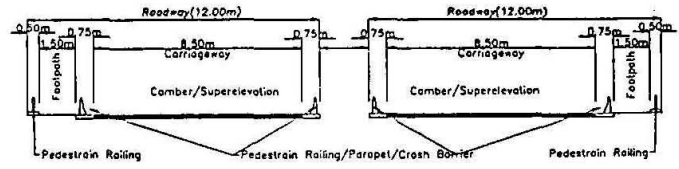
Cross Section of Bridge at Deck Level - With Footpath (Slab/Box type with open foundations) 4-LANE DIVIDED HIGHWAY Fig : 7.2A
