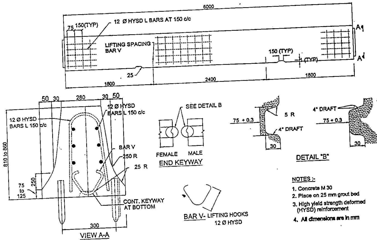
Fig. 9.6. ROAD SIDE BARRIER PRECAST DESIGN
