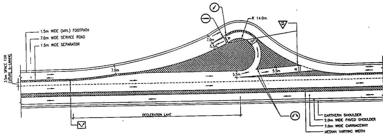
SUGGESTIVE LAYOUT FOR EXIT RAMP FROM HIGHWAY (SERVICE ROAD ON BOTH SIDES OF EXIT RAMP) FIG. 2.1D
