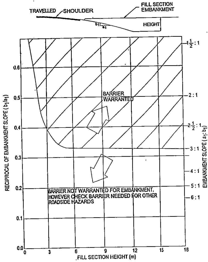
Fig. 9.1. WARRANTS FOR ROADSIDE BARRIERS ON EMBANKMENTS
