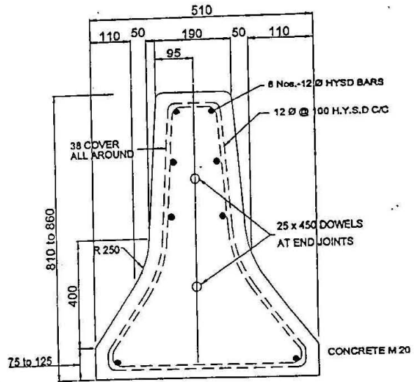
Fig. 9.11. MEDIAN BARRIER CAST-IN-SITU DESIGN
