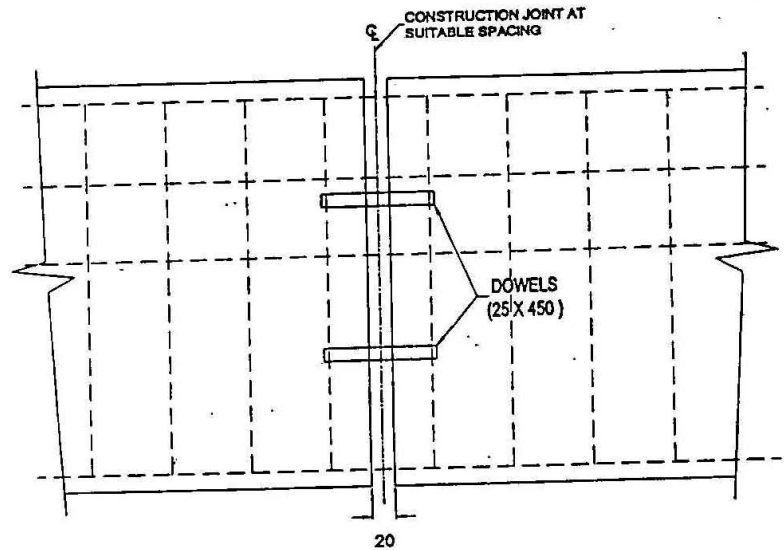
Fig. 9.11. MEDIAN BARRIER CAST-IN-SITU DESIGN
