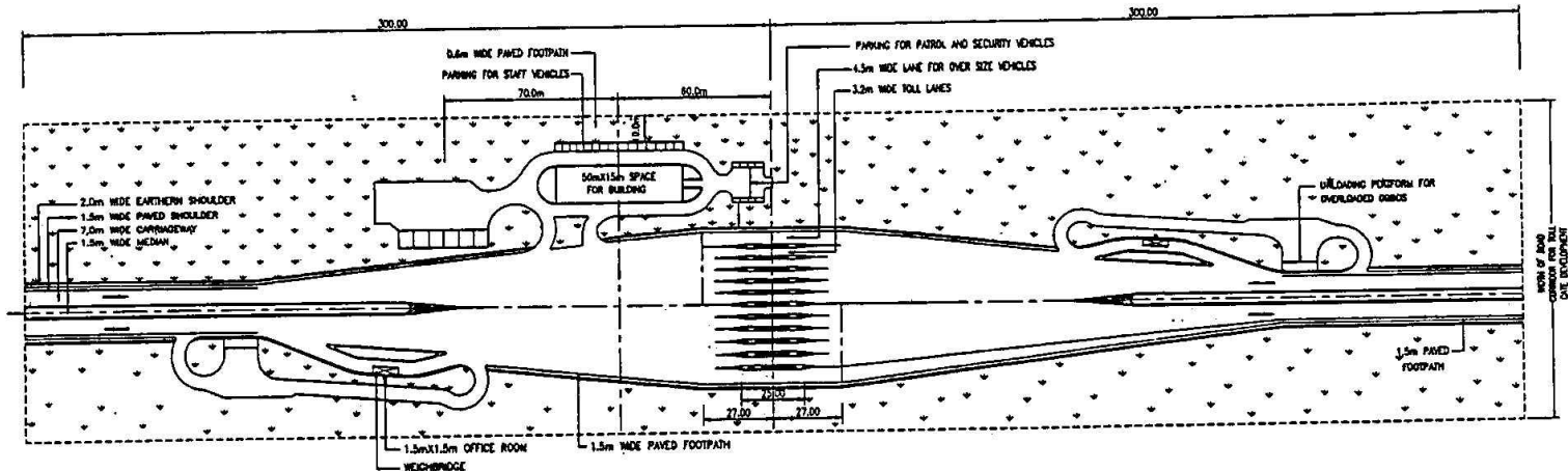
TYPICAL LAYOUT FOR A TOLL PLAZA
