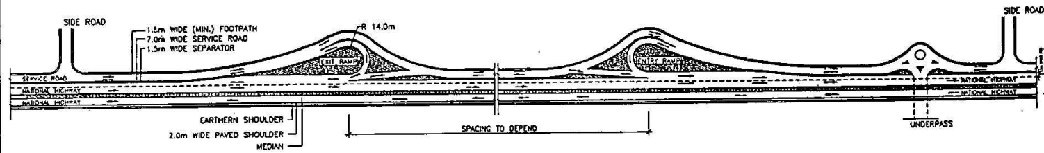
SUGGESTIVE LAYOUT SHOWING CONFIGURATION OF SERVICE ROAD, ENTRY/EXIT RAMP, SIDE ROAD AND UNDERPASS FIG. 2.1F
