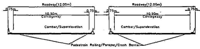
Cross Section of Bridge at Deck Level - Without Footpath (Slab/Box type with open foundations) 4-LANE DIVIDED HIGHWAY Fig : 7.2B
