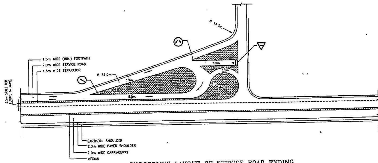
SUGGESTIVE LAYOUT OF SERVICE ROAD ENDING AT A JUNCTION WITH CROSS ROAD
