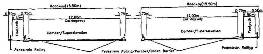
Cross Section of Bridge at Deck Level - With Footpath (T-Beam/Box Girder type/Well/Pile foundation) 4-LANE DIVIDED HIGHWAY ( Both side new Bridges)
